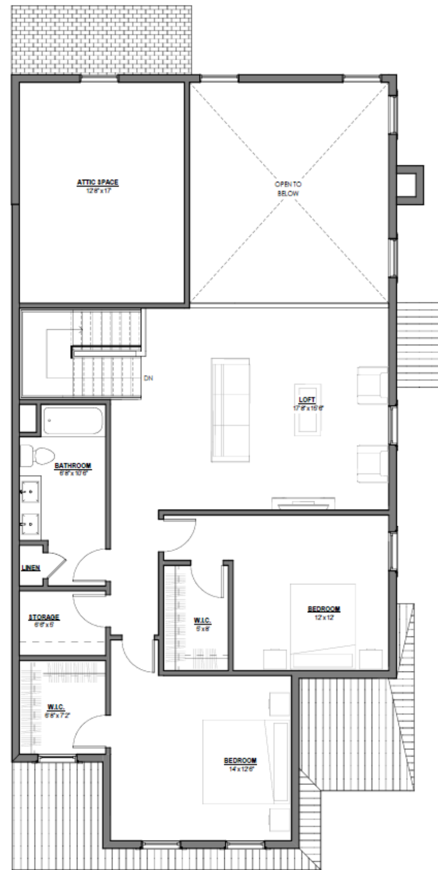
STANDARD SECOND FLOOR PLAN
