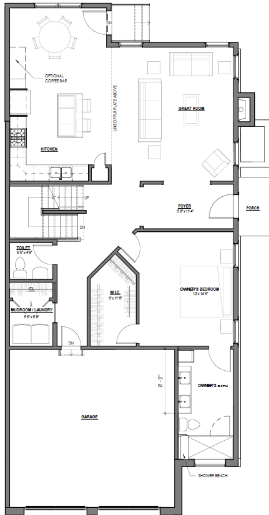
STANDARD FIRST FLOOR PLAN
