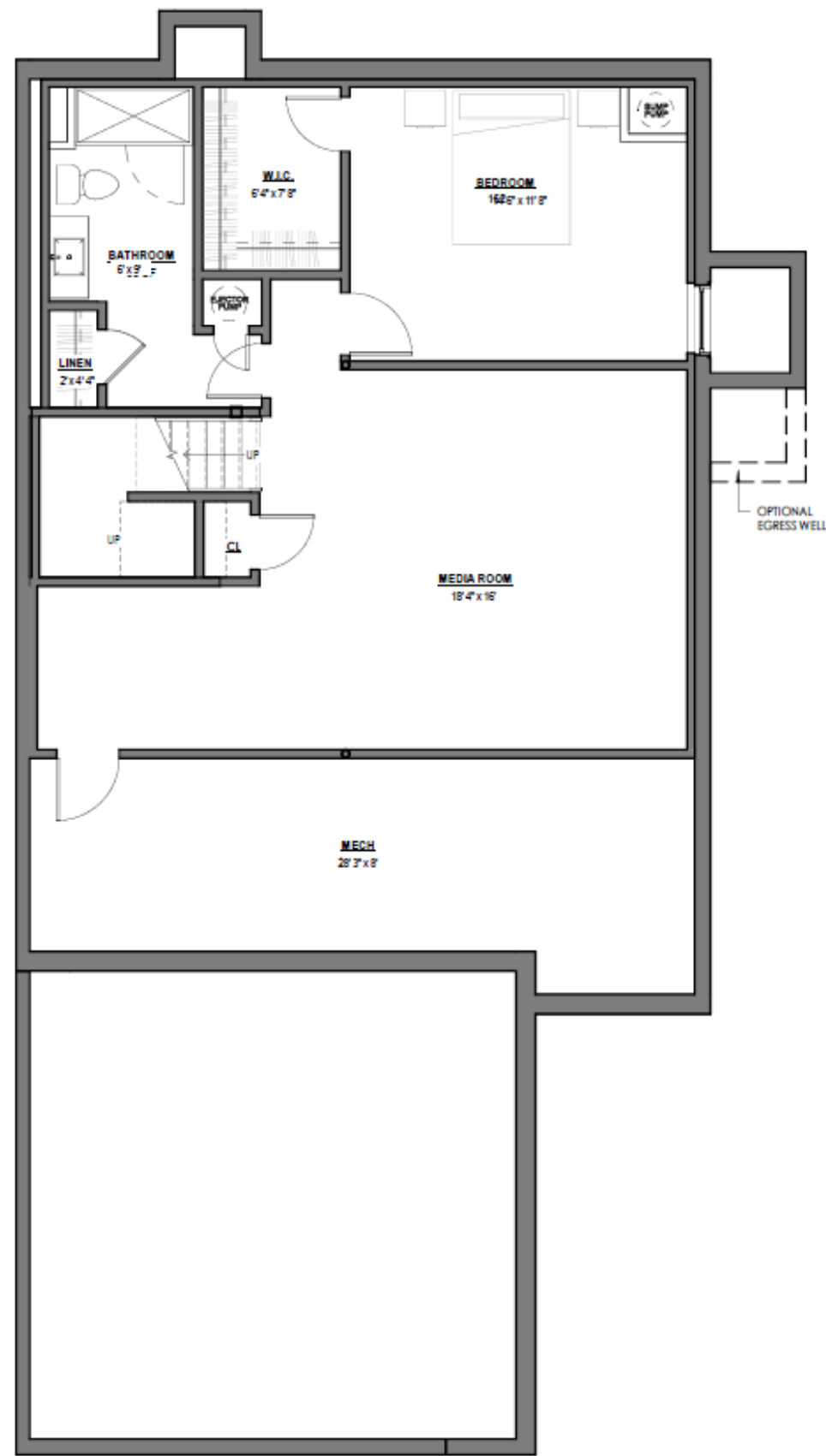
OPTIONAL BASEMENT FLOOR PLAN
