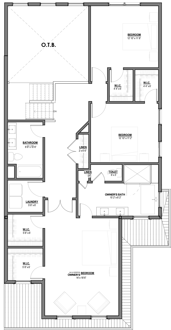
STANDARD SECOND FLOOR PLAN
