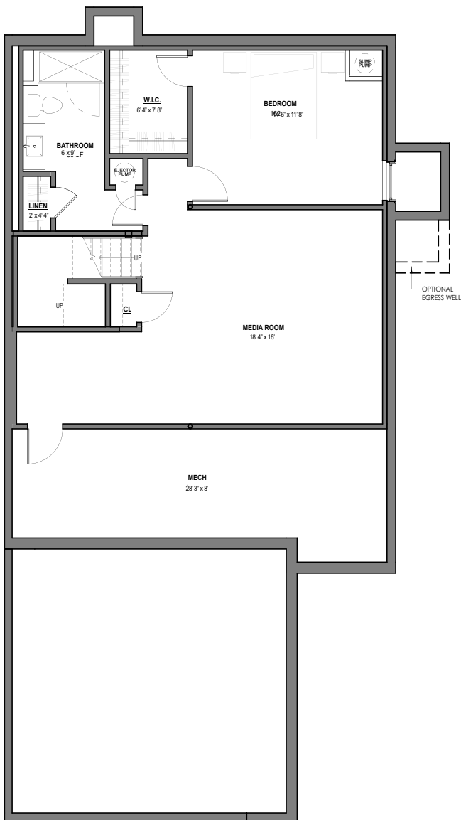
OPTIONAL BASEMENT FLOOR PLAN
